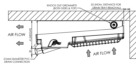
SIDE ELEVATION
