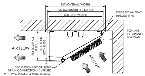
SIDE ELEVATION
